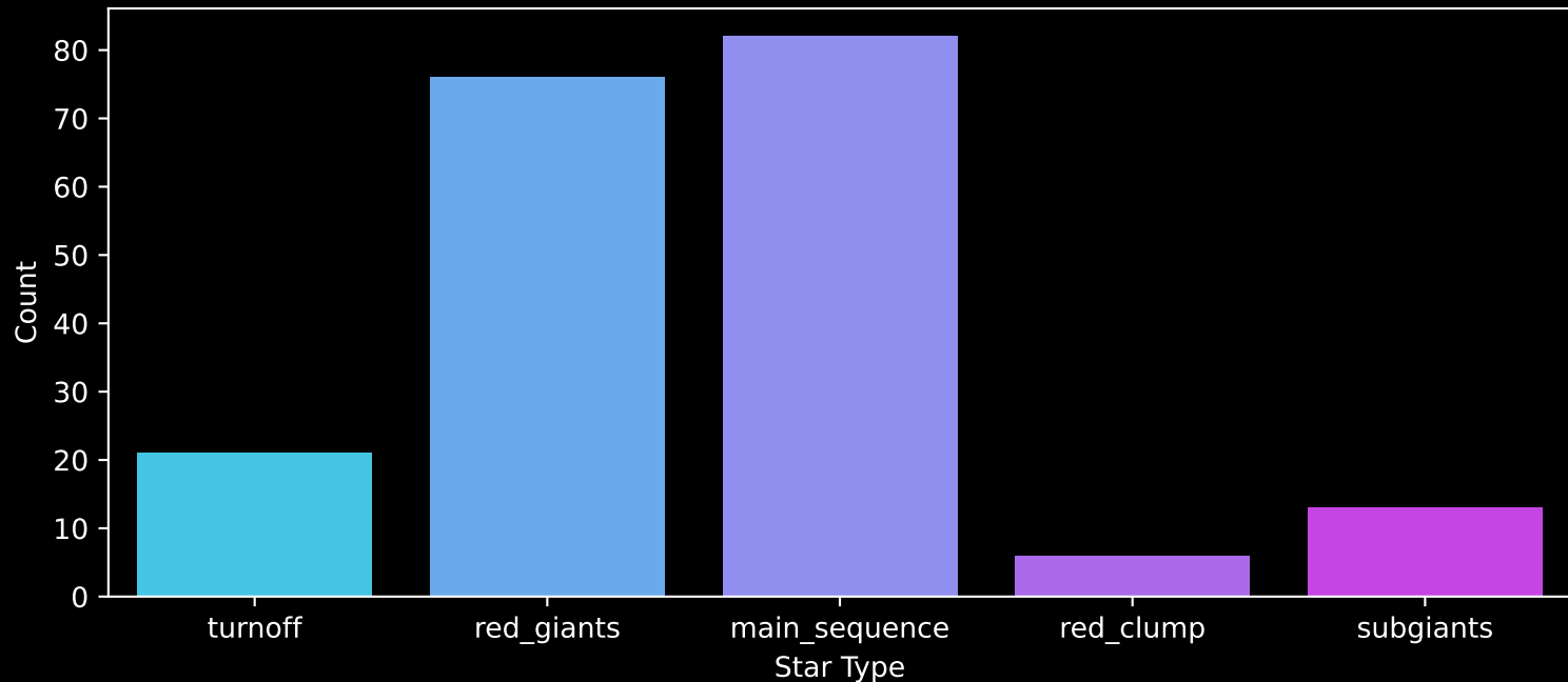
APOGEE DR17 Field: [165-45] Count plot of Star Type
