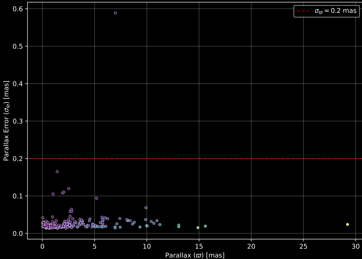
APOGEE DR17 Field: [165-45] Parallax Quality (n= 198)
