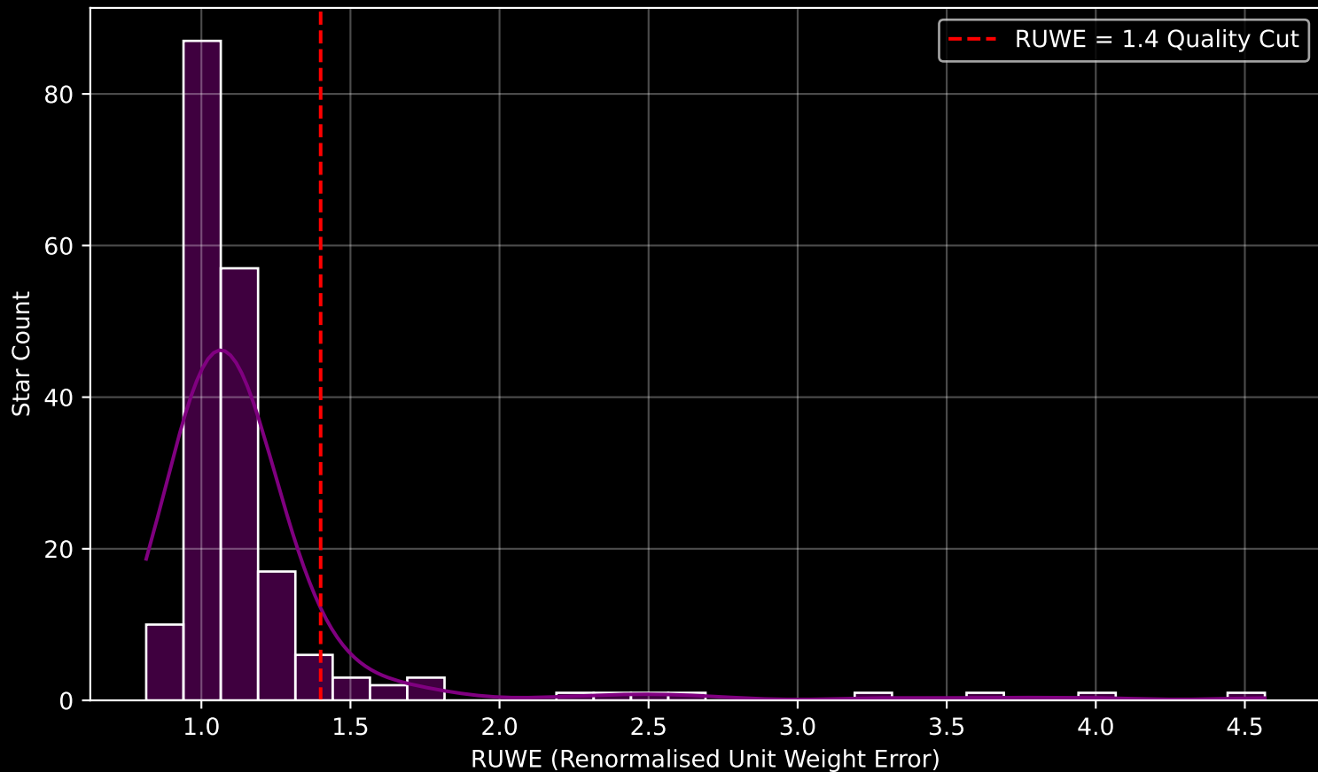
GAPOGEE DR17 Field [165-45] RUWE Distribution (n= 193)
