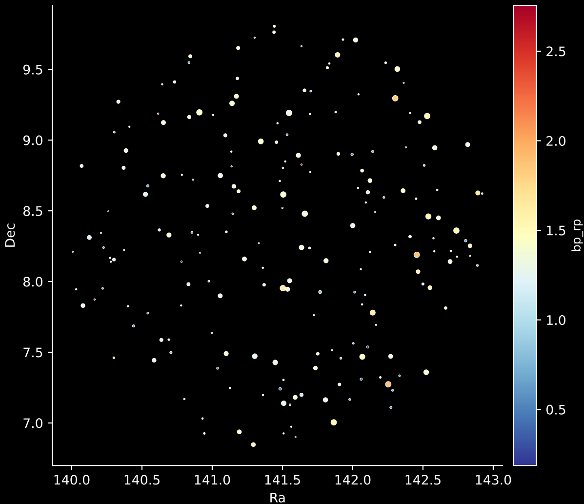
APOGEE DR17 Field: [165-45] Stars: 198
