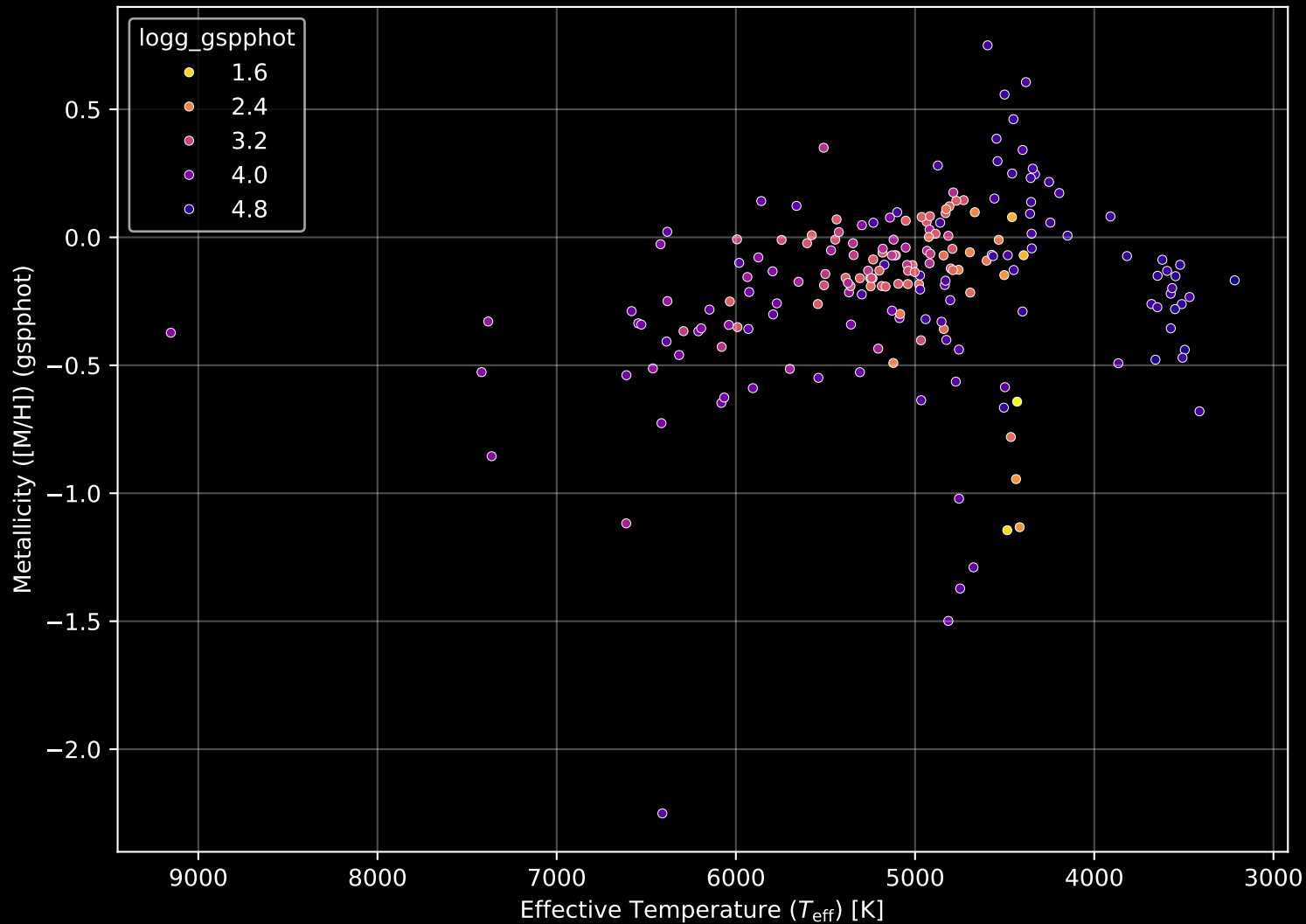
APOGEE DR17 Field: [165-45] Stellar Population Parameters (n= 198)
