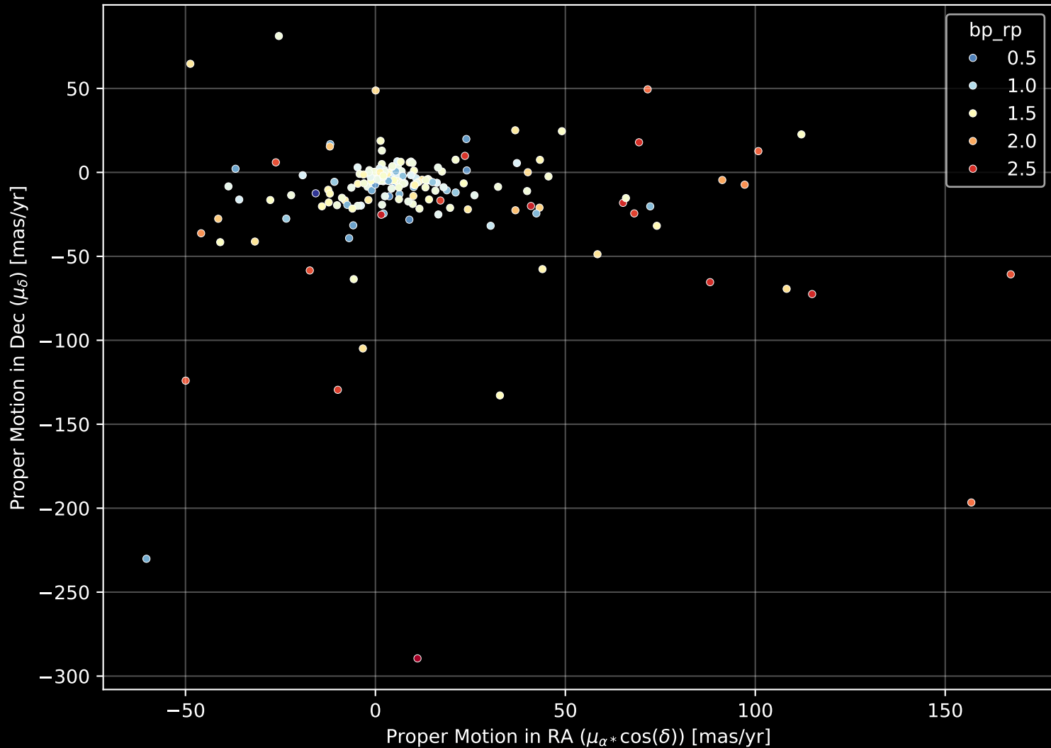
APOGEE DR17 Field: [165-45] Proper Motion Diagram (n= 198)
