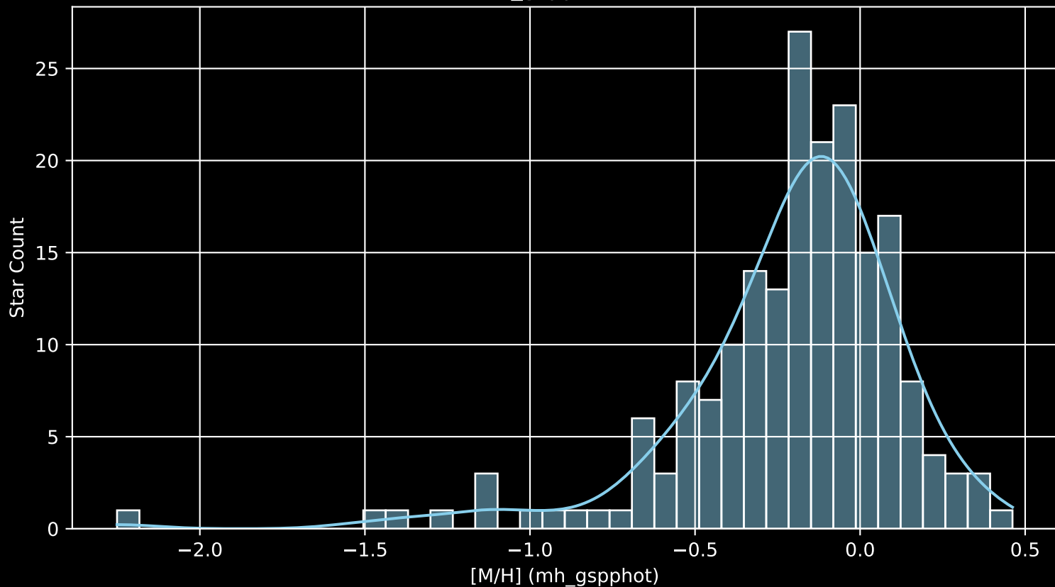
APOGEE DR17 Field: [165-45 [M/H] (mh_gspphot) (n= 195)
